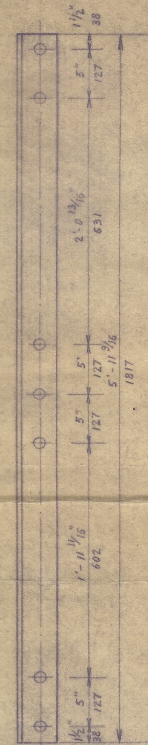
Pos 18 L 4x4 3/8 x 5x11 1/2
