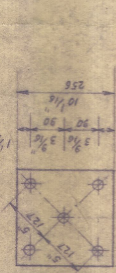
Pos 25 L 4x4 3/8 x 5x11 1/2
