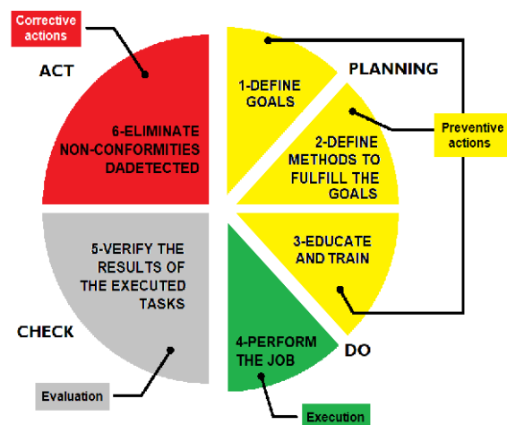
Figure 1. PDCA Cycle (3)
