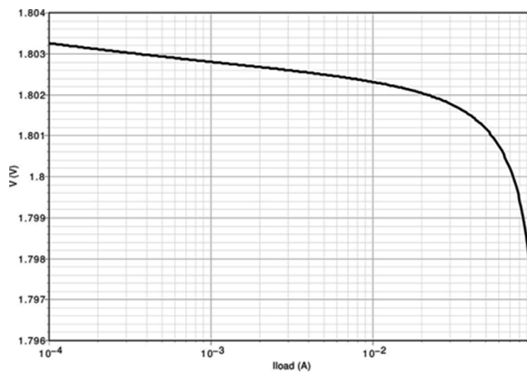
Figure 7. Load regulation.
