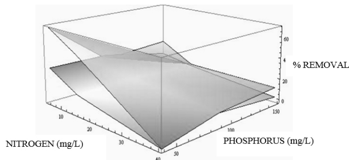
Figure 3. Phosphorus removal by darkness trial (bottom sheet) and lighted trial (top sheet).
