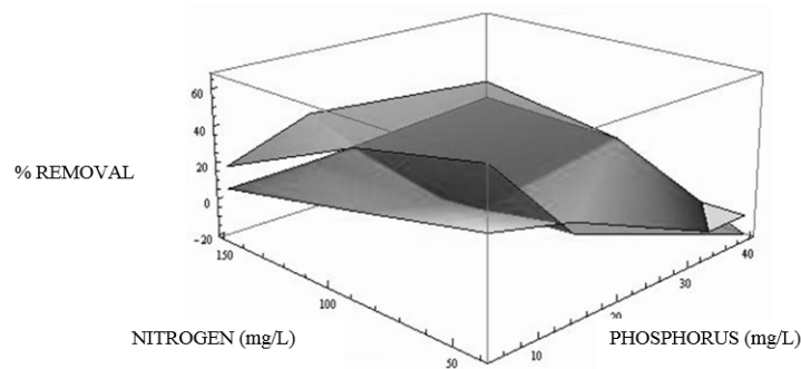
Figure 2. Nitrogen removal by darkness trial (bottom sheet) and lighted trial (top sheet).
