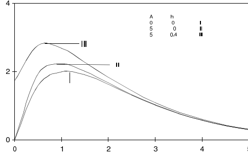
Figure 2: The velocity profiles of carbon dioxide ( Sc = 0.94 ) in air ( Pr = 0.71 ) for Gr = 2 , Gc = 2 , \omega t = 0 , \omega = 10 and \epsilon = 0.2 .
