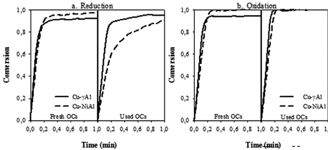
Figure 4. Solid conversion vs. time curves in TGA for a) reduction and b) oxidation reactions of fresh and after-used Cu-based OCs particles. Reduction: \text{CH}_4 = 15\% , \text{H}_2\text{O} = 20\% , \text{N}_2 = 65\% . Oxidation: air. T = 1073 \text{ K} . Cu- \gamma\text{Al} . Cu-NiAl.
