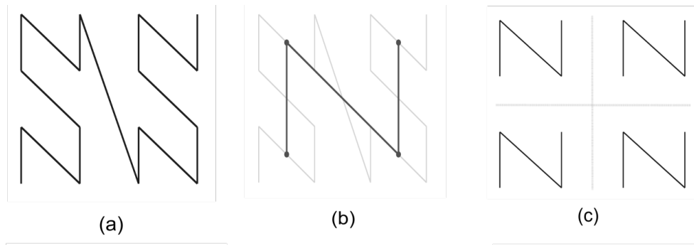
Figure 12. Self-Similarity Test for Lebesgue curve.
