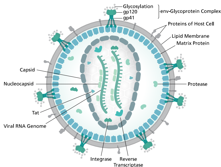
Figure 2: HIV-1 Proteome.
