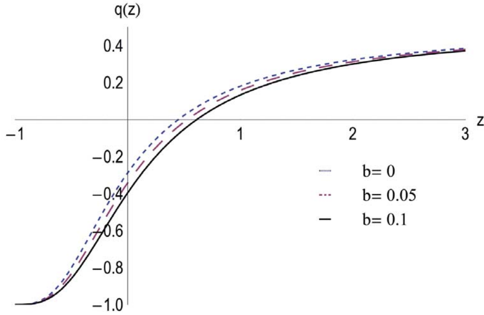
Figure 2: Plot of the deceleration parameter q versus the redshift z , using suitable values for the coupling constant b .
