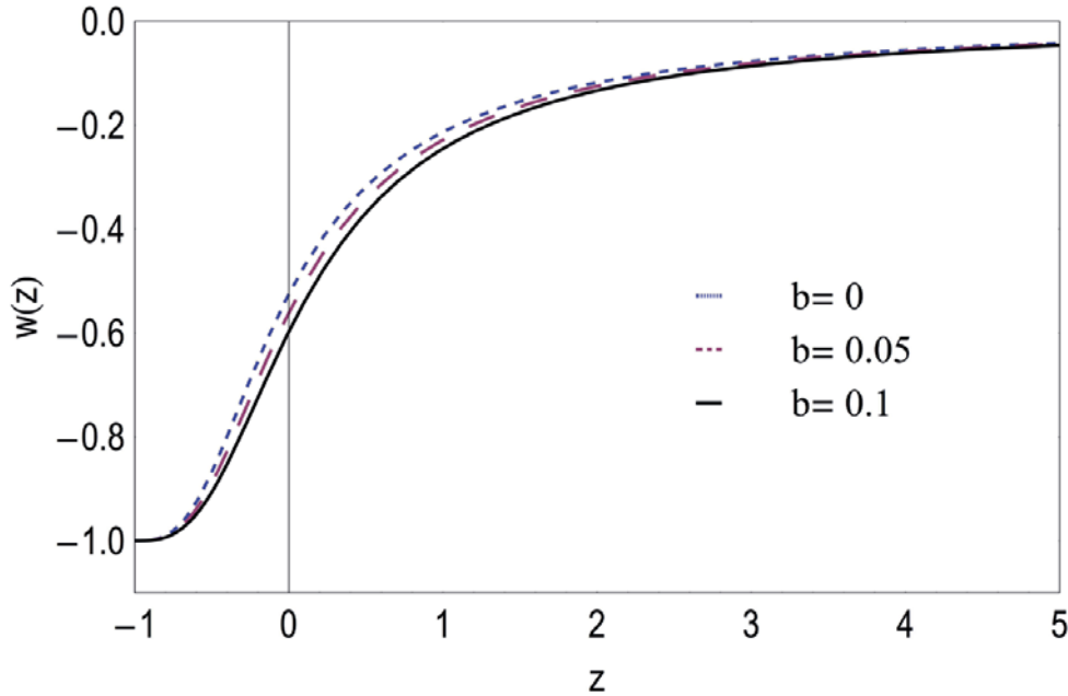
Figure 1: Plot of the equation of state parameter w versus the redshift z , using suitable values for the coupling constant b .
