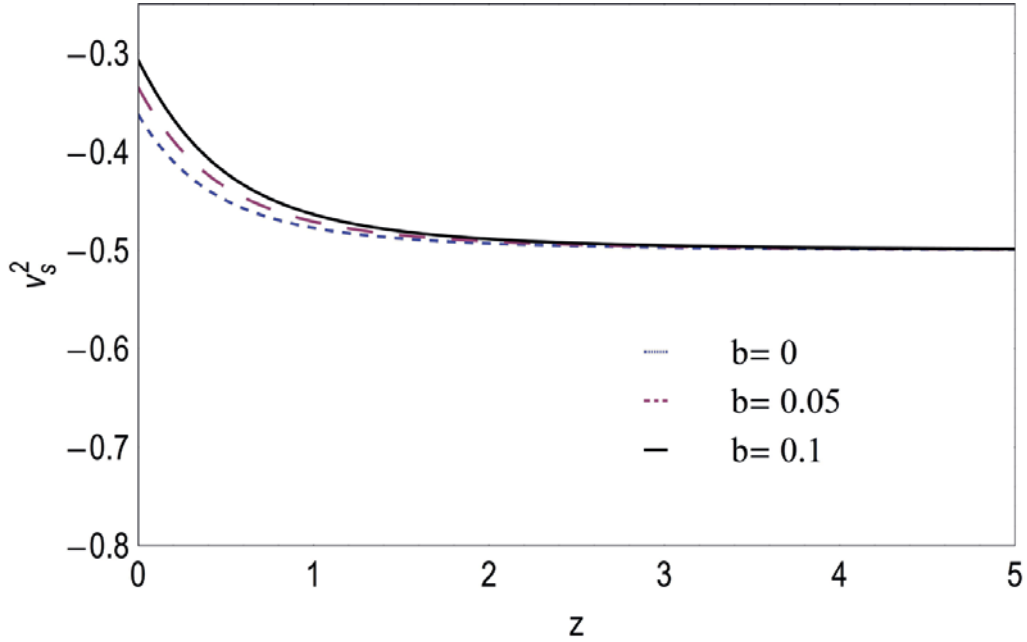
Figure 3: Plot of the square of the velocity of sound v_s^2 versus the redshift z , using suitable values for the coupling constant b .
