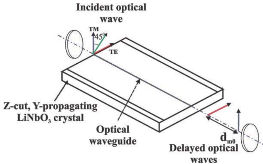
Figure 1. An optical waveguide on a \text{LiNbO}_3 substrate working as optical retarder.
