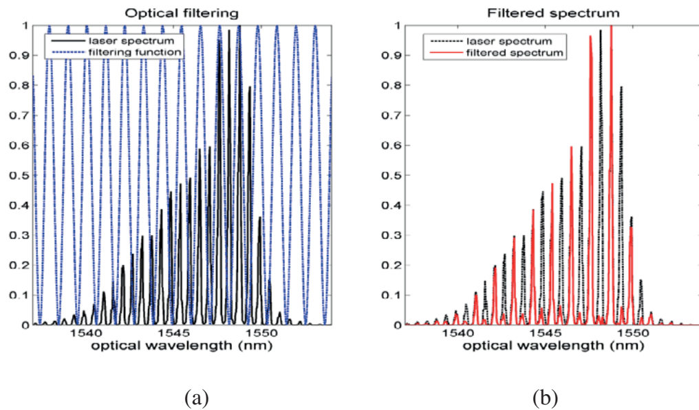
Figure 5. a) The multimode unfiltered optical spectrum; b) the filtered optical spectrum.
