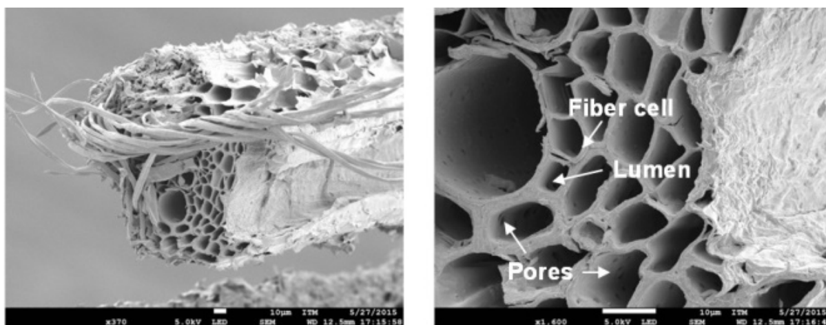
Figure 3. SEM micrographs of untreated pineapple leaf fiber.
