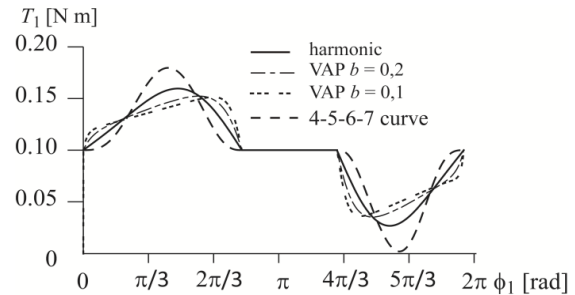
Figure 12. Input torques.
