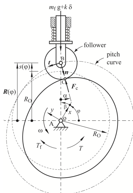
Figure 6. Cam profile.
