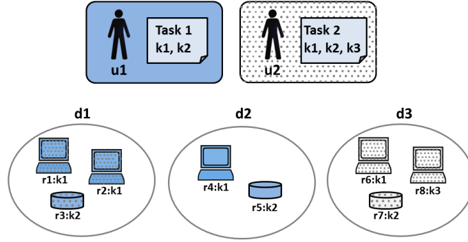
Figure 2 A GC Scenario: Two users ( u_1, u_2 ), two VO ( v_1 – blue, v_2 – dotted), three ADs ( d_1, d_2, d_3 )
