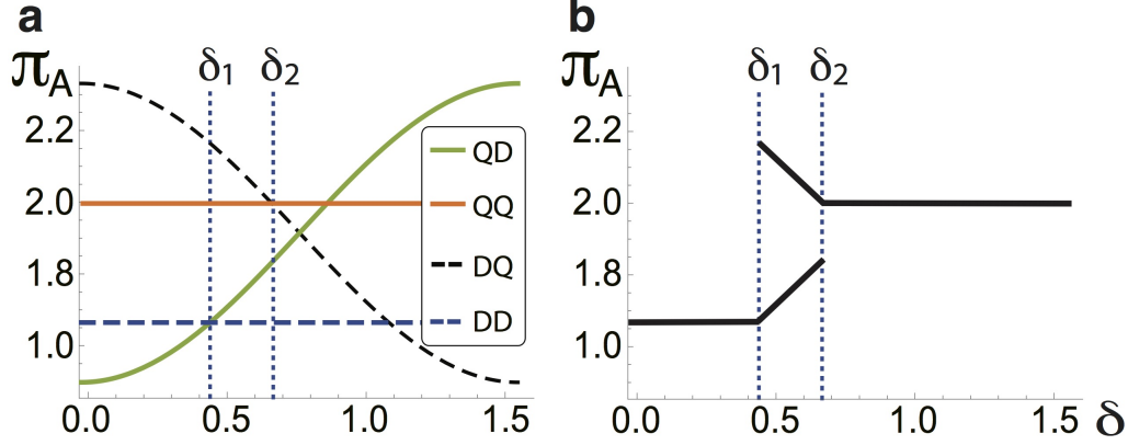
Figure 35: Payoffs for general states \rho_{in}(p, \delta) : (a) the control of the initial state correlations, and \tilde{\mathcal{J}}(\delta) imply thresholds at \delta_1 = \sin^{-1} \sqrt{1/5} , and \delta_2 = \sin^{-1} \sqrt{2/5} , (b) strategies reaching the Nash equilibrium in the regions defined by \delta_1 and \delta_2 .
