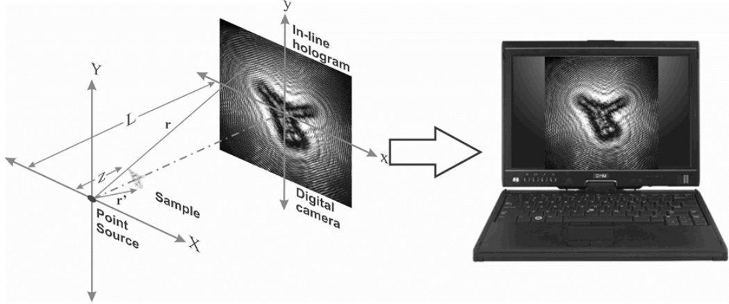
Figure 1. Recording stage in digital lensless holographic microscopy (DLHM).
