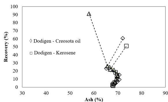
Figure 2. Release analysis curves obtained with Dodigen frother.
