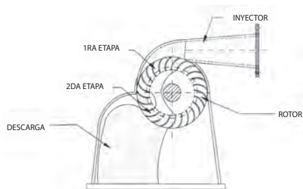
Figura 2.9 Turbina Michell [18]
