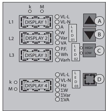
Figura 4.4 Panel frontal Lovato [37]
