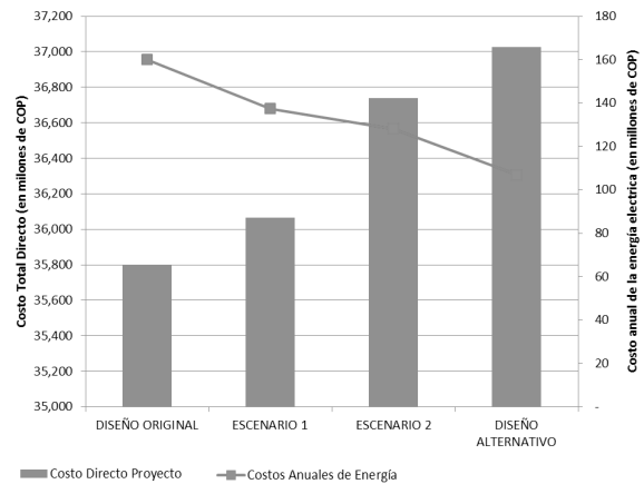
Figure 7. Direct cost of the project and annual electrical energy cost for each analyzed case.
