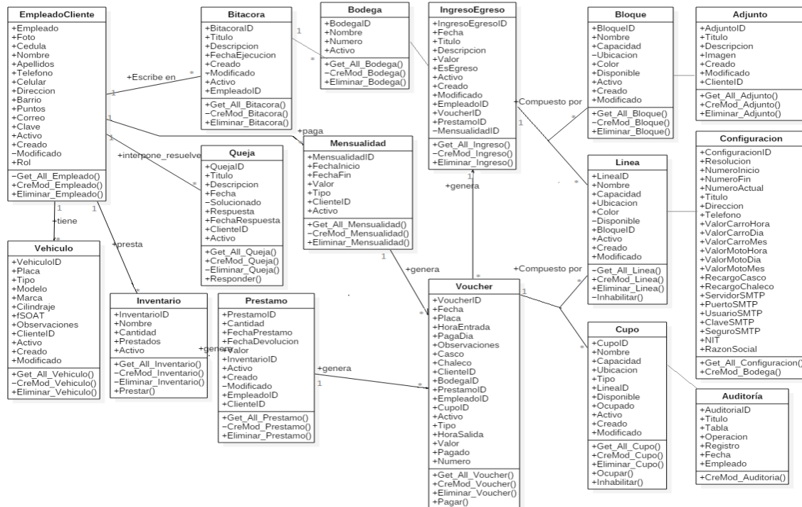
Figure 2. Class diagram
