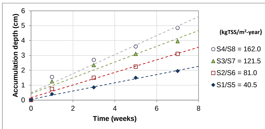
Figure 32 Accumulation trends at different SLRs
